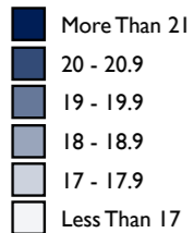
ACT Scores
