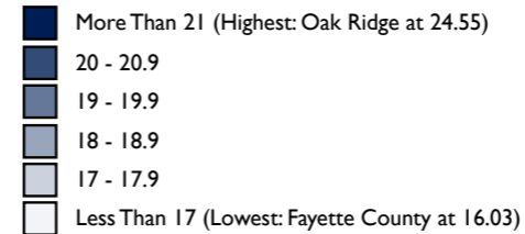
ACT Scores
